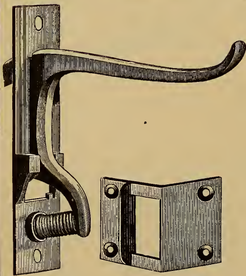
Half Size Cut of Latch with Nos. 35 and 45.
