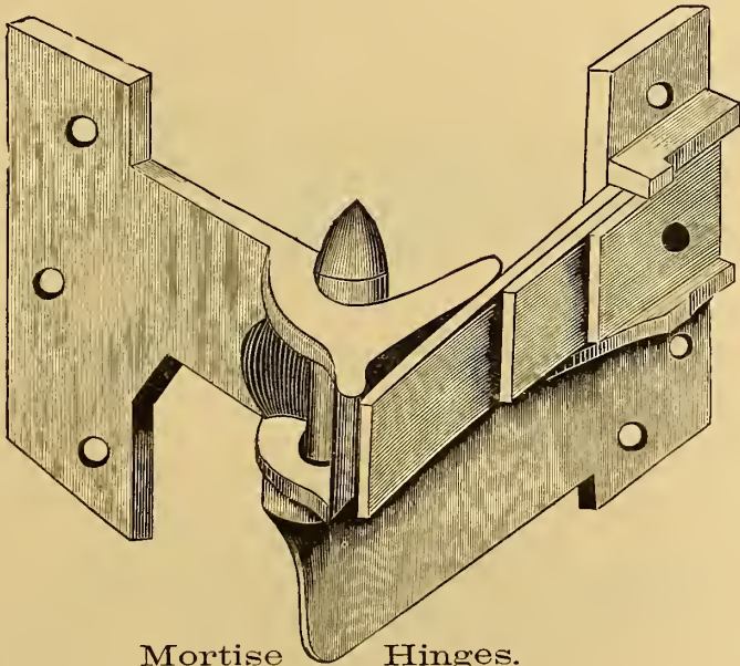
Mortise Hinges.
