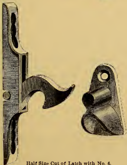
Half Size Cut of Latch with No. 6.
