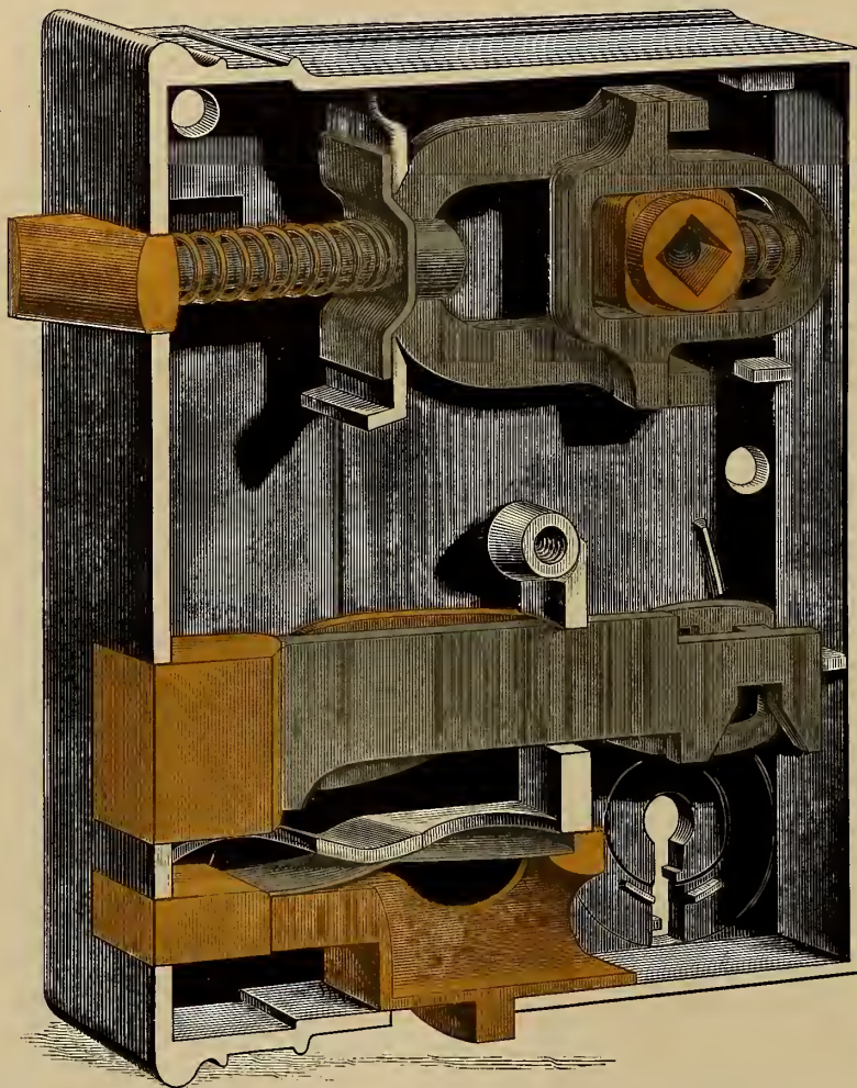
INTERIOR VIEW OF THE "BUILDERS'" LOCK.
