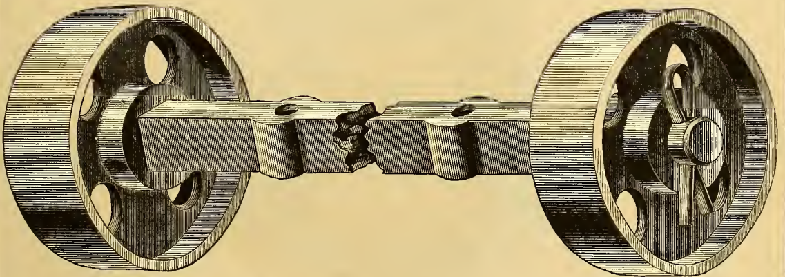
No. 874. Half Size Cut with piece of Axle cut out,
