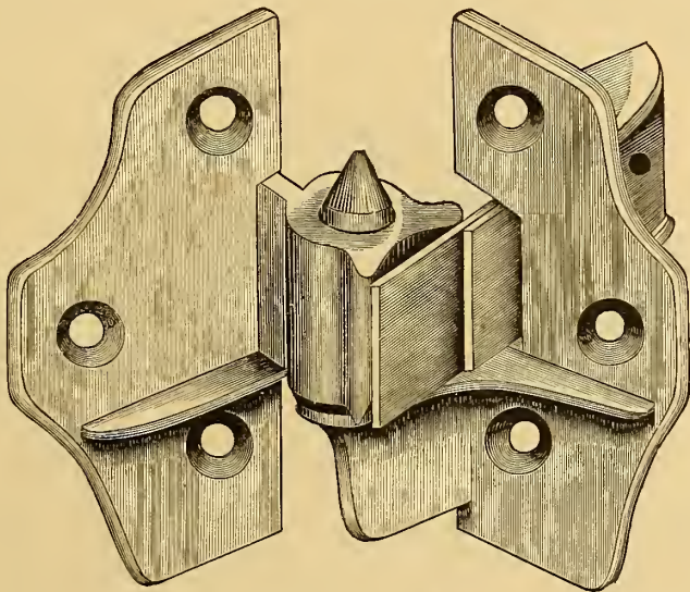
Surface Hinges.
